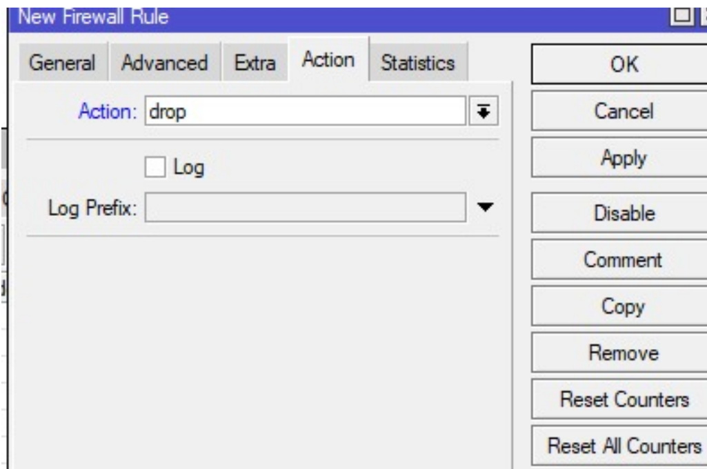
Gambar 15: action
