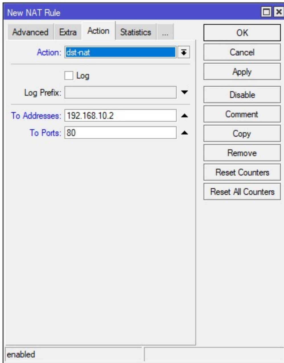
Gambar 20: action
