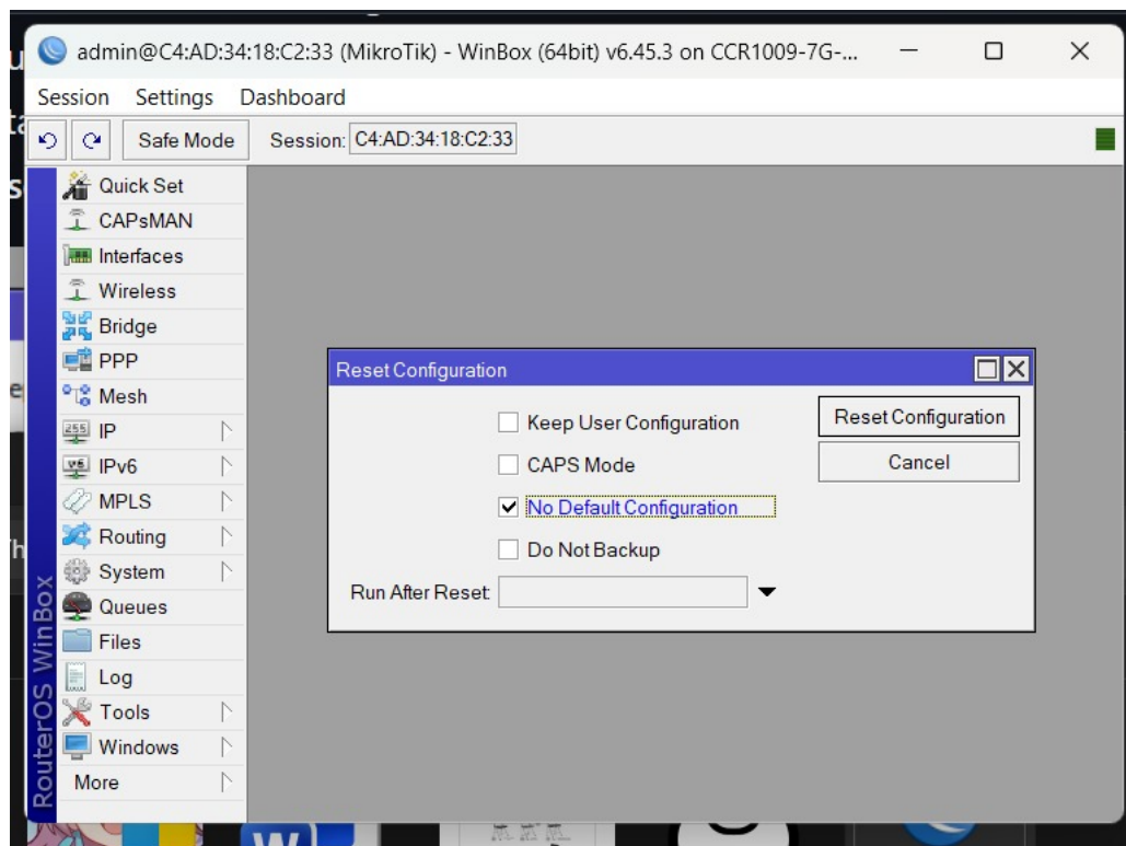
Gambar 1: reset configuration
