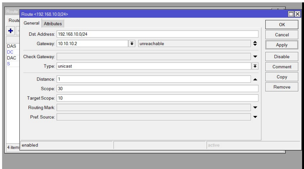
Gambar 5: static routing
