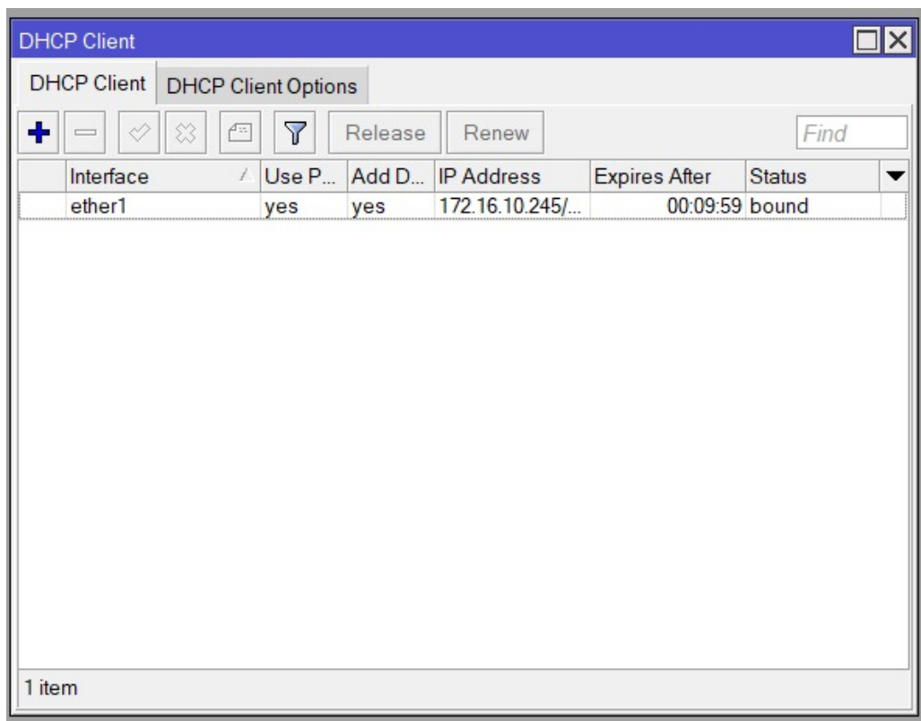
Gambar 8: dhcp client
