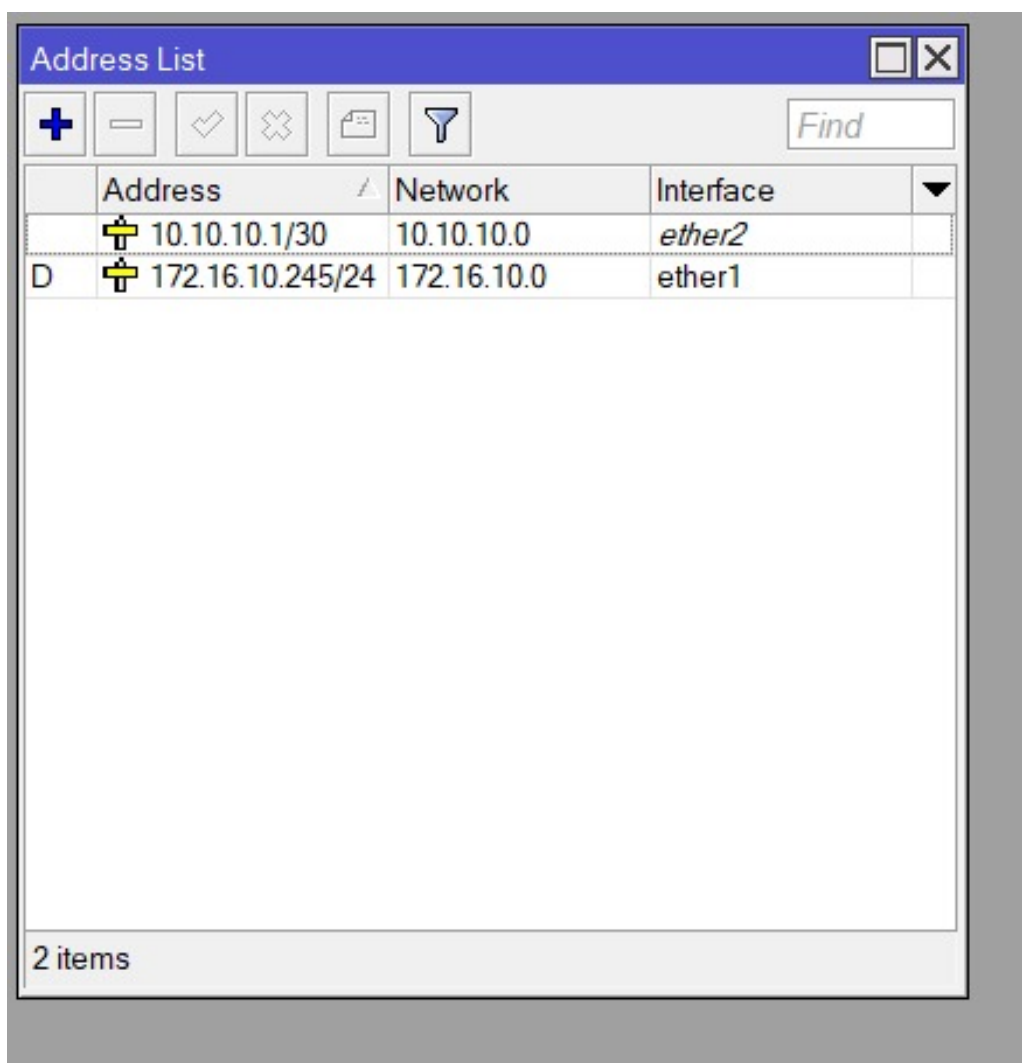
Gambar 6: IP
