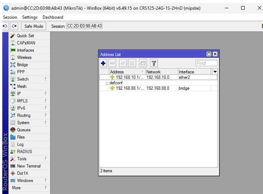
Gambar 9: ip address
