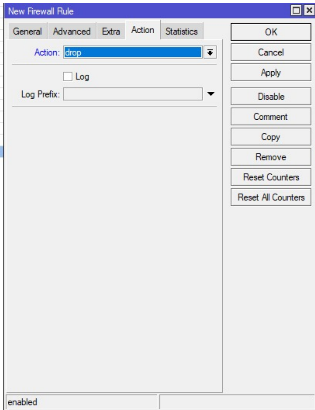
Gambar 18: action drop
