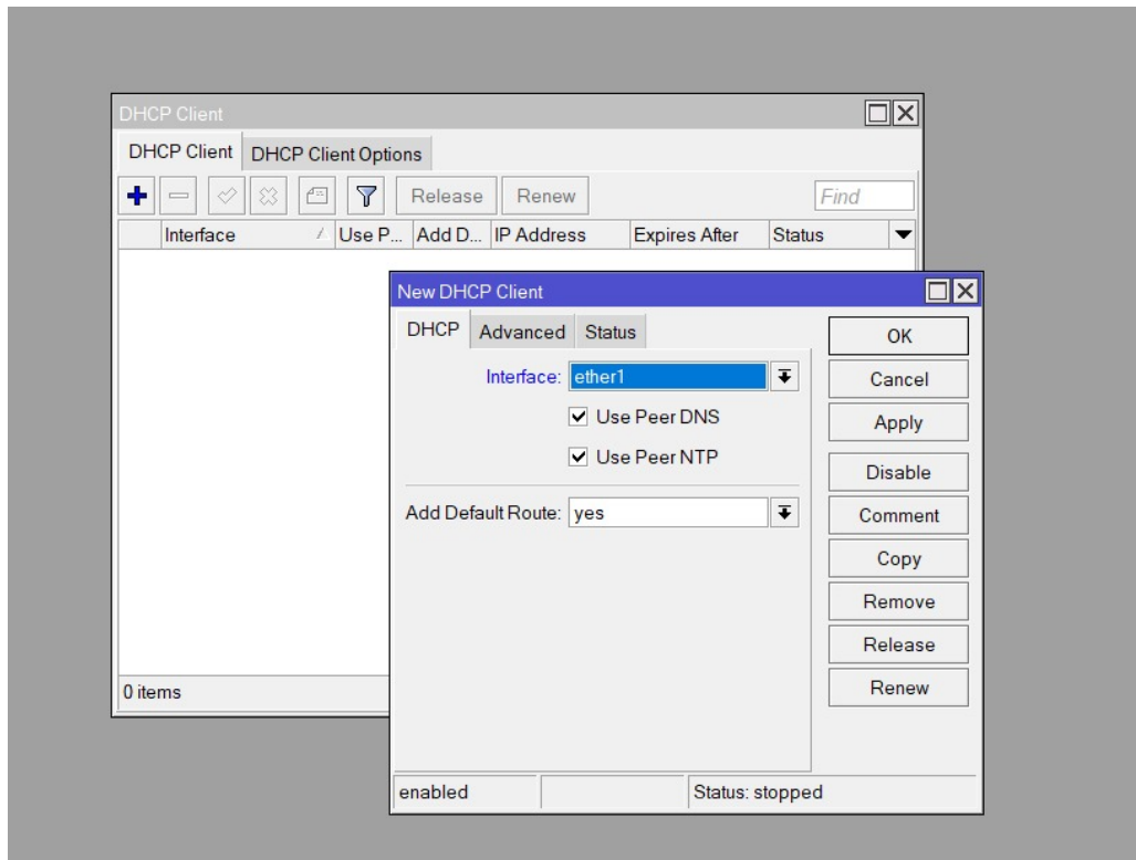
Gambar 7: set dhcp
