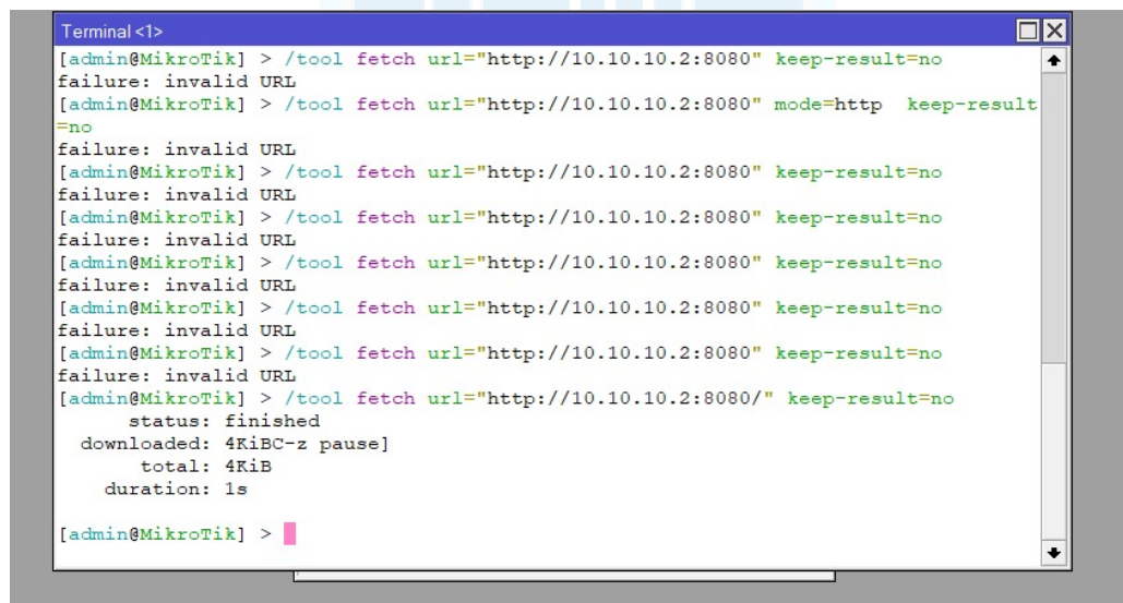
Gambar 2: fetch url
